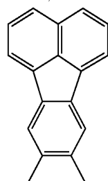
8,9-FlAn
