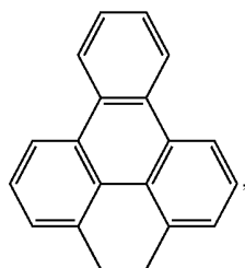
1,12-TriP
