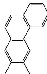
2,3-PhAn
