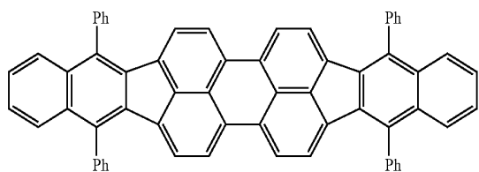
Red 2
