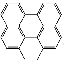
1,12-Per
