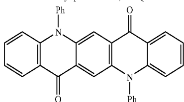
Diphenylquinacridone, DPQA
