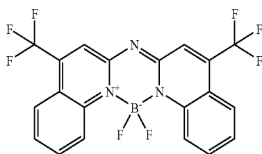
ADPMB 1
