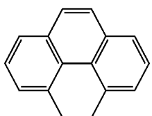
4,5-PhAn
