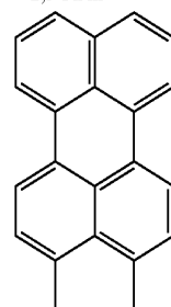
3,4-Per
