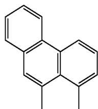
1,10-PhAn
