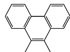
9,10-PhAn
