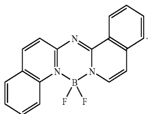
ADPMB 2
