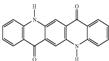
Quinacridone, QA
