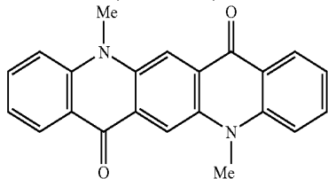
Dimethylquinacridone, DMQA
