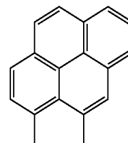
1,10-Pyr
